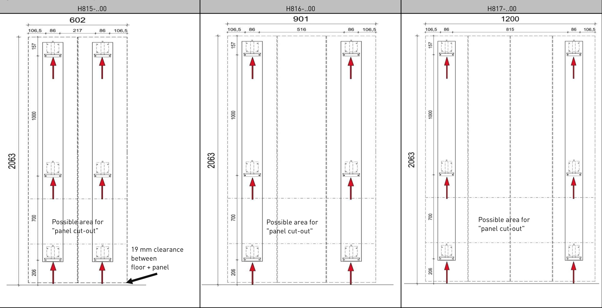
Fig. 4: Drill dimensions for suspension rails
